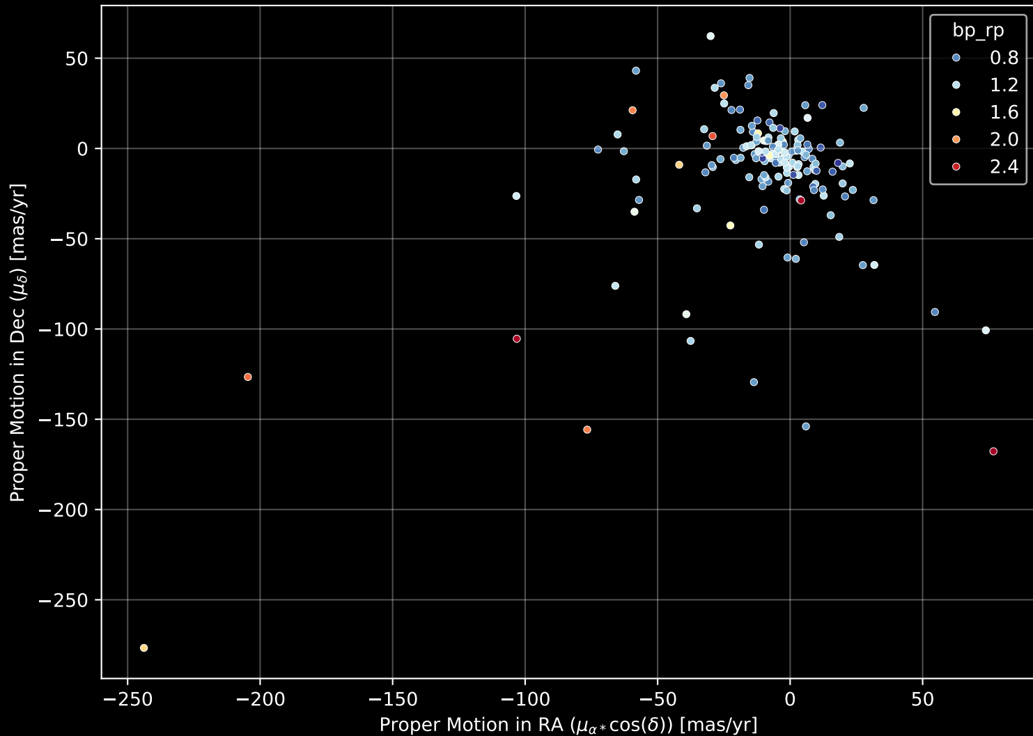
APOGEE DR17 Field: [046+45_MGA] Proper Motion Diagram (n= 164)
