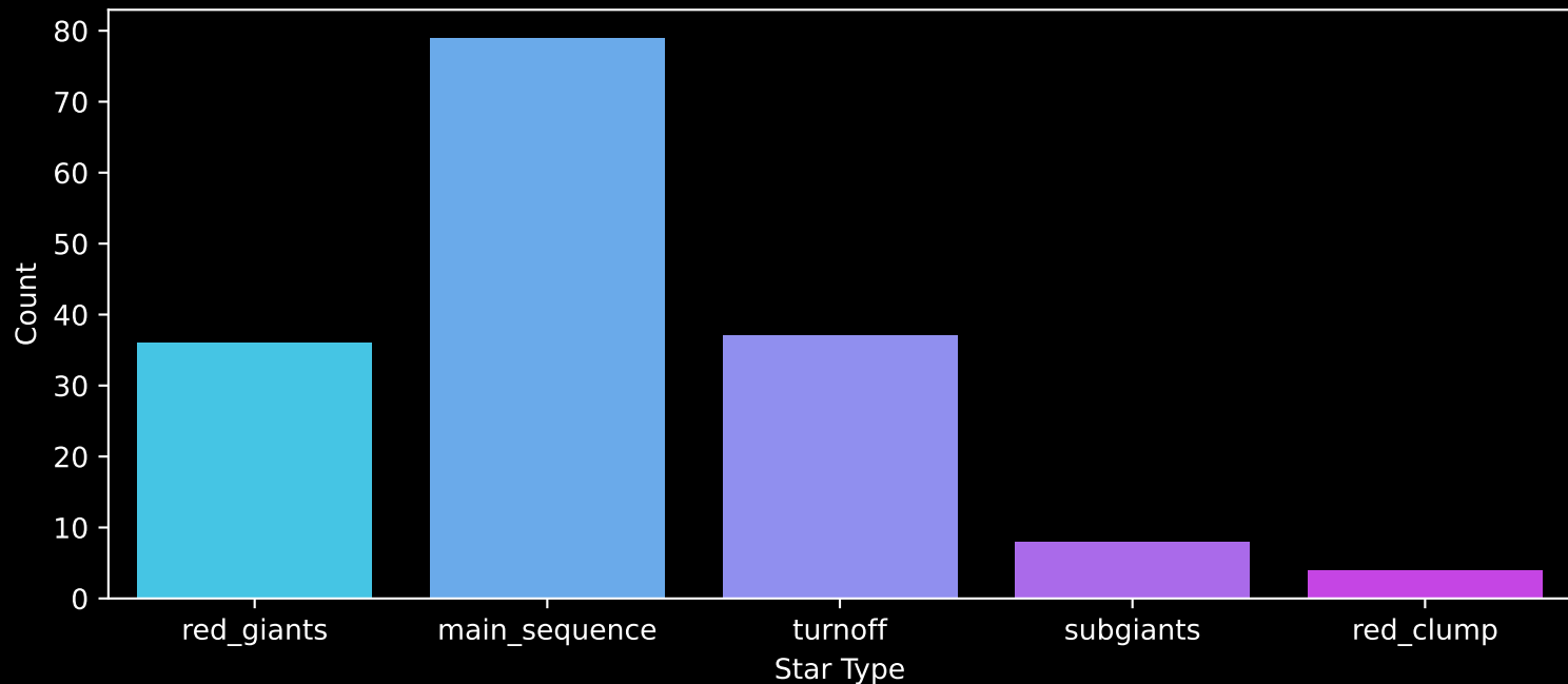
APOGEE DR17 Field: [046+45_MGA] Count plot of Star Type
