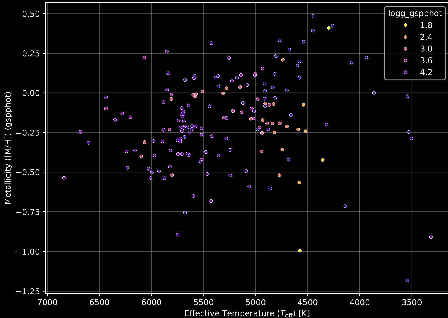
APOGEE DR17 Field: [046+45_MGA] Stellar Population Parameters (n= 164)
