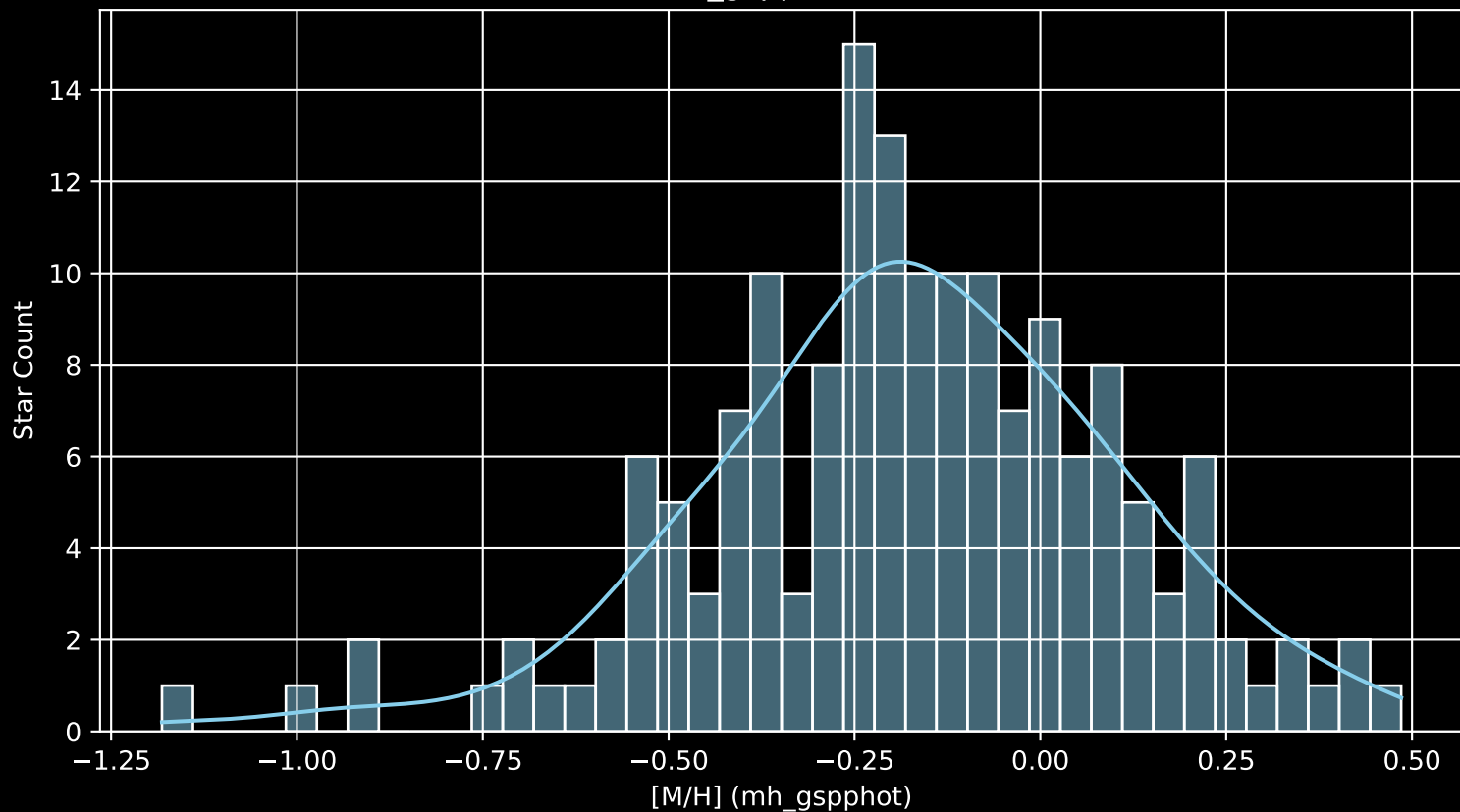
APOGEE DR17 Field: [046+45_MGA [M/H] (mh_gspphot) (n= 164)
