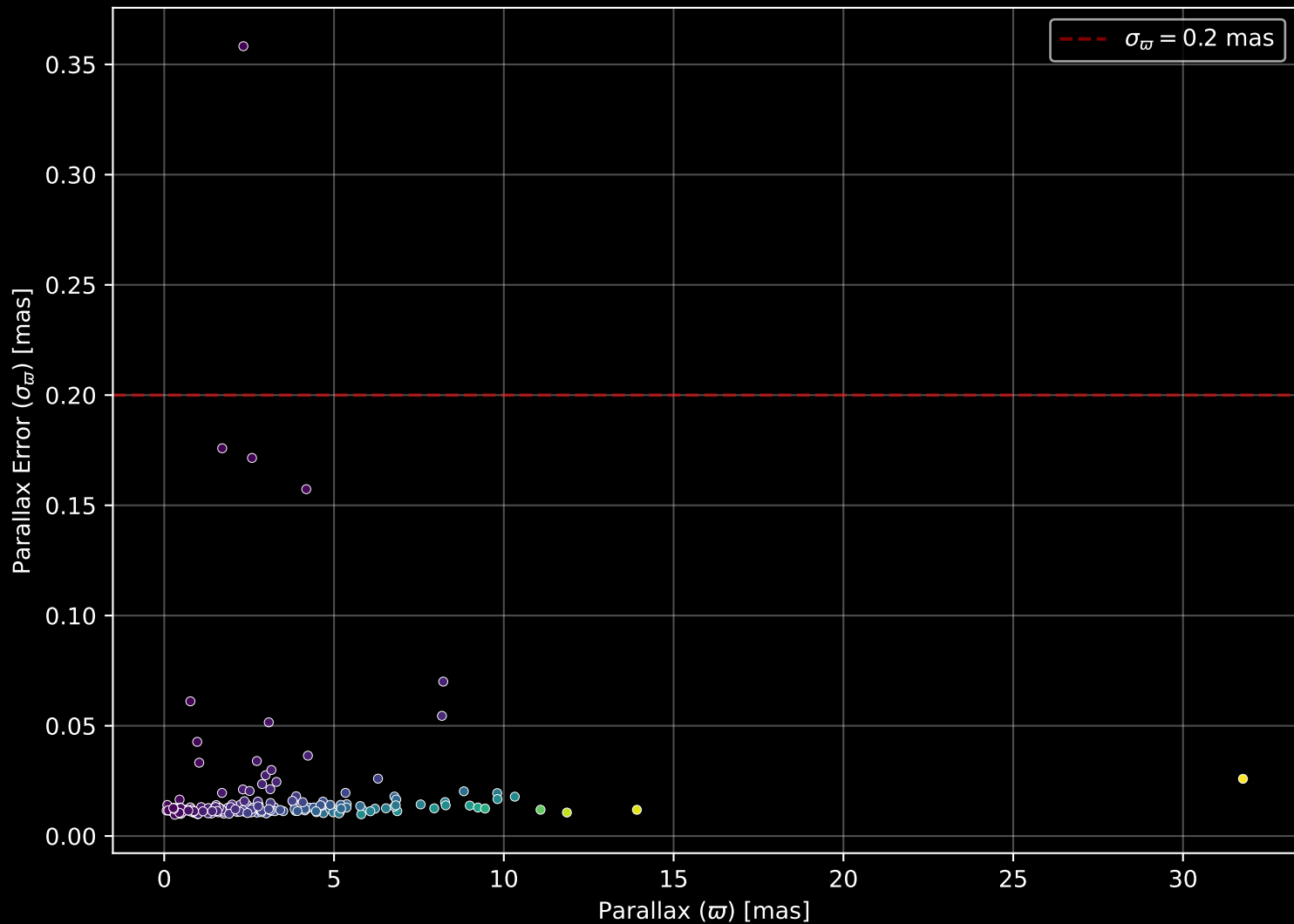
APOGEE DR17 Field: [046+45_MGA] Parallax Quality (n= 164)
