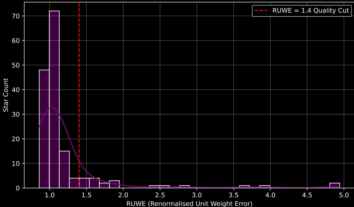
GAPOGEE DR17 Field [046+45_MGA] RUWE Distribution (n= 159)
